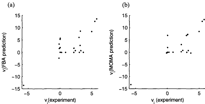
Fig. 1. Intracellular flux determination for mutant strain \Delta zwf . Units for both axes are millimoles per gram dry weight per hour ( \text{mmol/gDW/h} ). (a) FBA flux predictions for the mutant do not correlate well with experimental measurements. (b) MOMA predictions are expected to better correlate with experimental fluxes. However, in this case, even MOMA predicted mutant fluxes are not satisfactory enough for inferring biomass coefficients.
